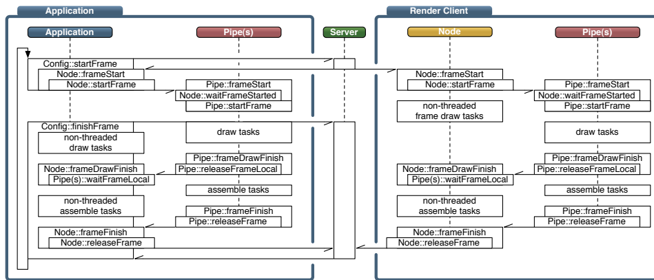
Figure 39: Synchronization of Frame Tasks
