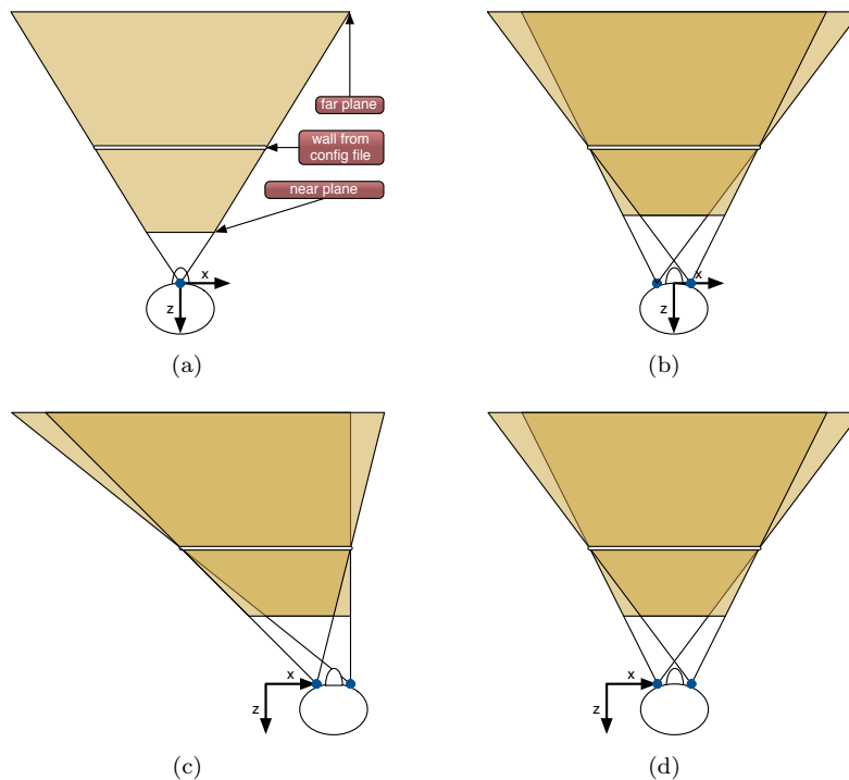
Figure 40: Monoscopic (a), Stereoscopic (b), Tracked (c) and HMD (d) Frusta
