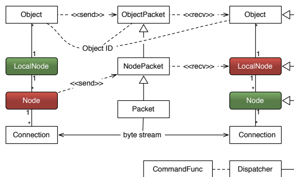
Figure 56: Communication between two Objects
