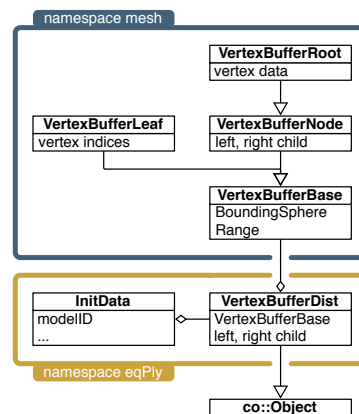
Figure 28: Scene Data in eqPly
