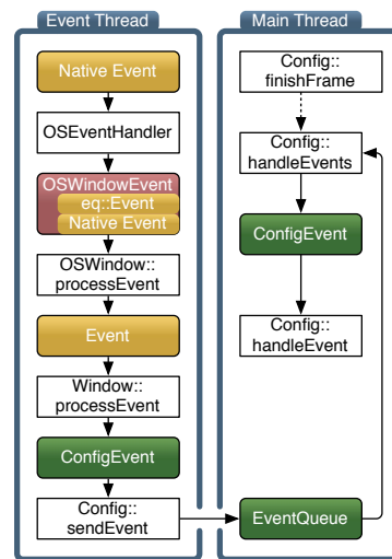
Figure 34: Event Processing
