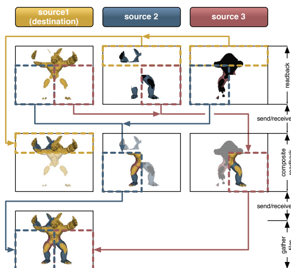
Figure 44: Direct Send Compositing
