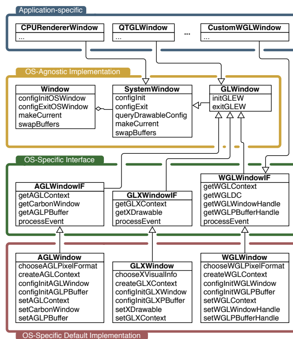
Figure 31: SystemWindow UML Class Hierarchy
