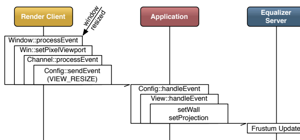
Figure 43: Event Flow during a View Update
