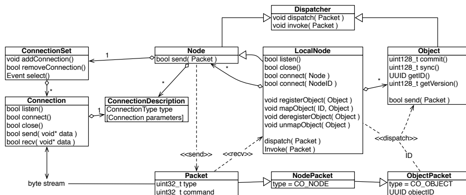
Figure 52: UML class diagram of the major Collage classes
