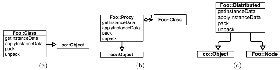
Figure 54: Object Distribution using Subclassing, Proxies or Multiple Inheritance
