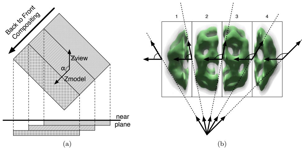
Figure 49: Back-to-Front Compositing for Orthogonal and Perspective Frusta
