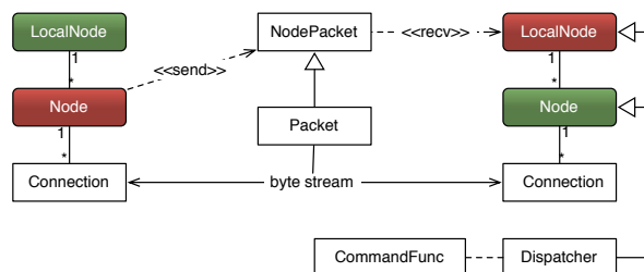
Figure 53: Communication between two Nodes
