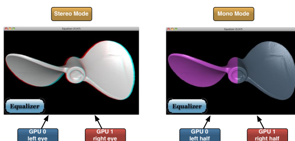
Figure 42: Using two different decompositions during stereo and mono rendering
