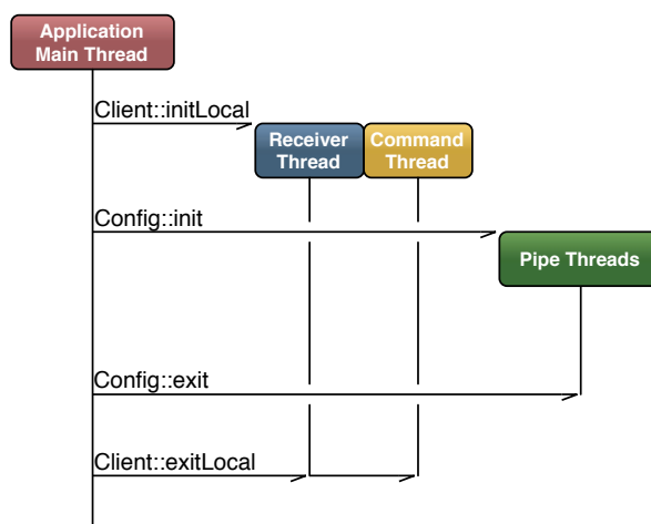
Figure 36: Threads within one Node Process
