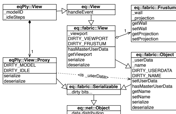
Figure 41: UML Hierarchy of eqPly::View
