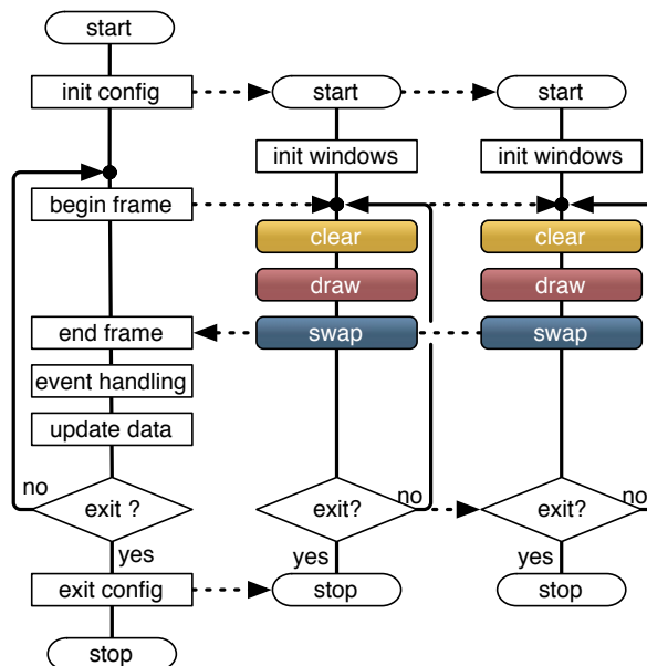
Figure 1: Parallel Rendering
