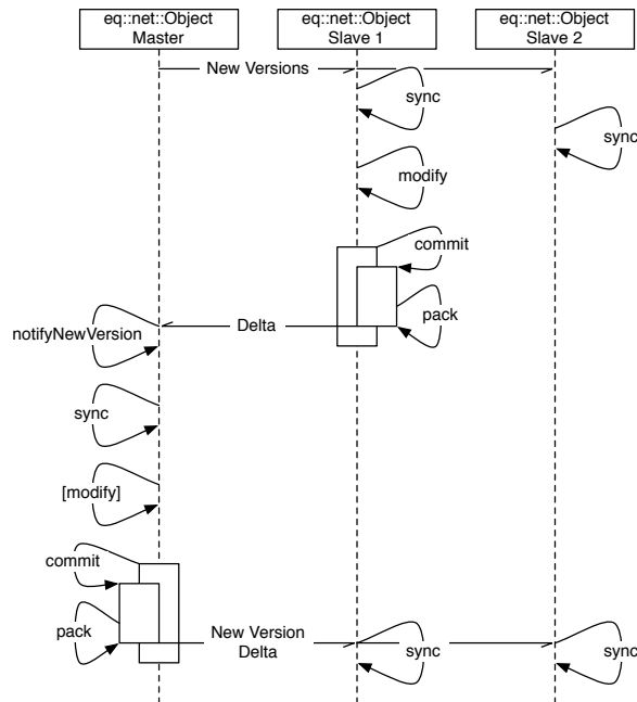
Figure 55: Slave Commit Communication Sequence
