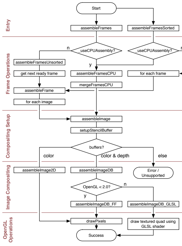
Figure 46: Functional Diagram of the Compositor
